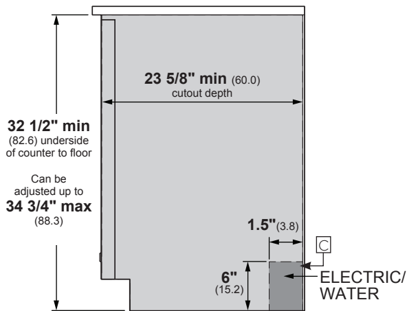
FLUSH CUTOUT INSTALLATION
