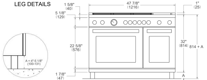
LEG DETAILS
