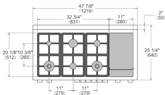
WORKTOP DETAILS
