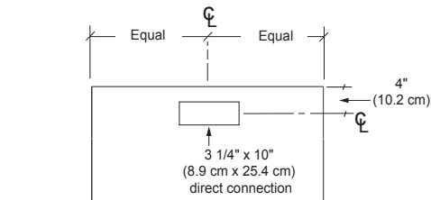
MICROWAVE EXHAUST LOCATION
