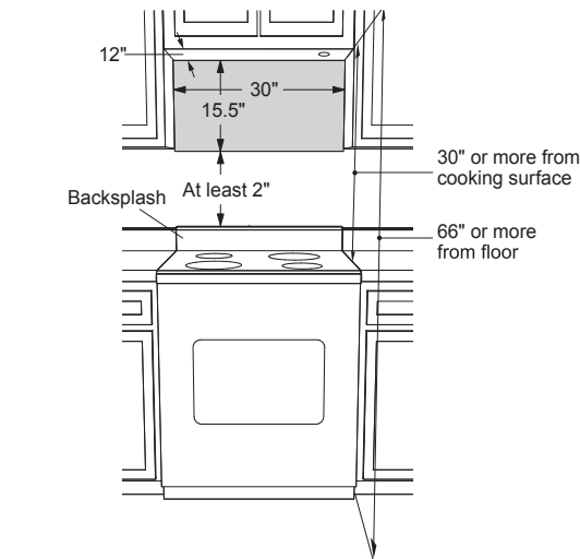
UPPER CABINET DIMENSIONS
