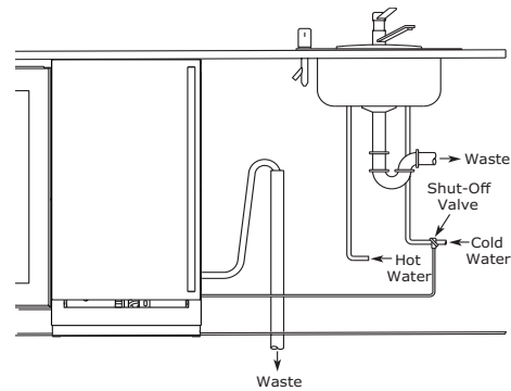
Disposal Assembly P60 Pump Required
