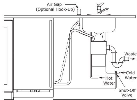
Y-Branch Tailpiece P60 Pump Required
