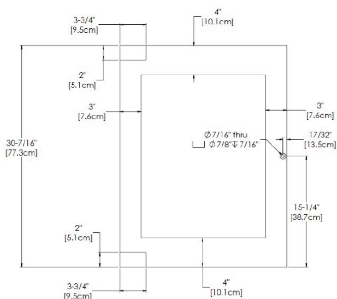
Right Hand Hinged Door 24" (61 cm) wide appliance
