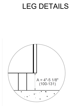
LEG DETAILS
